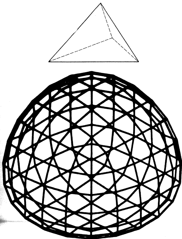
Figure 4. Original tetrahedron used to generate Figure 3 with line drawing of the generated surface
