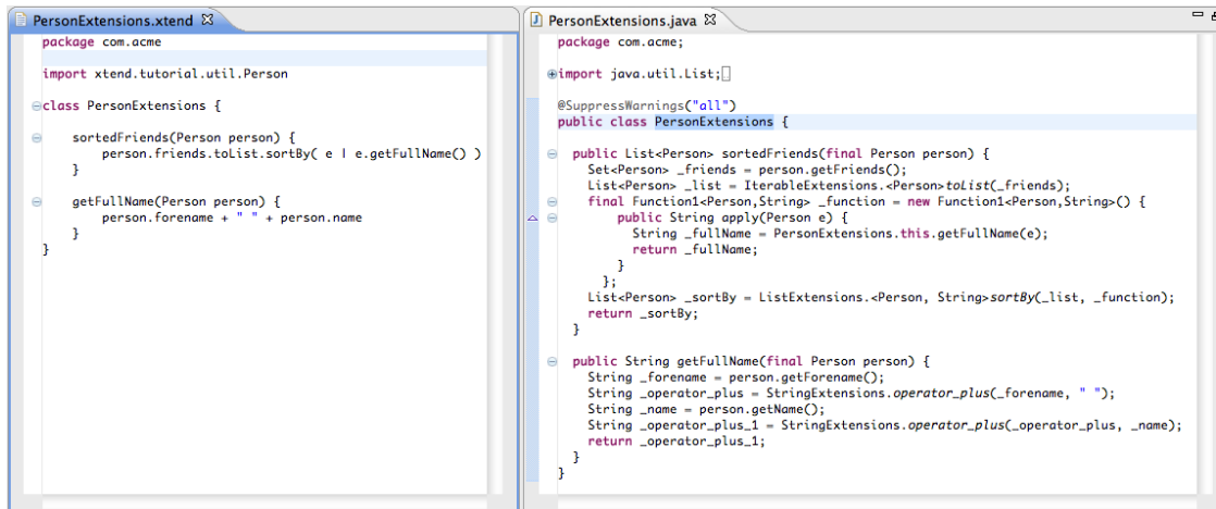
Figure 12.1.: Xtend and Java Vis-a-Vis
