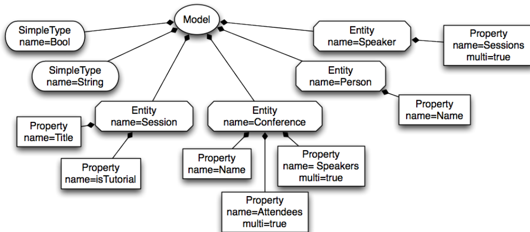
Figure 13.1.: Sample AST
