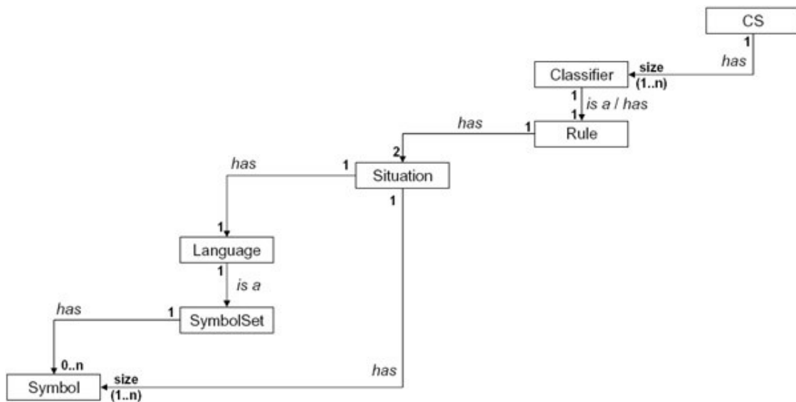
Figure 1. Simplified scheme of the library's main classes
