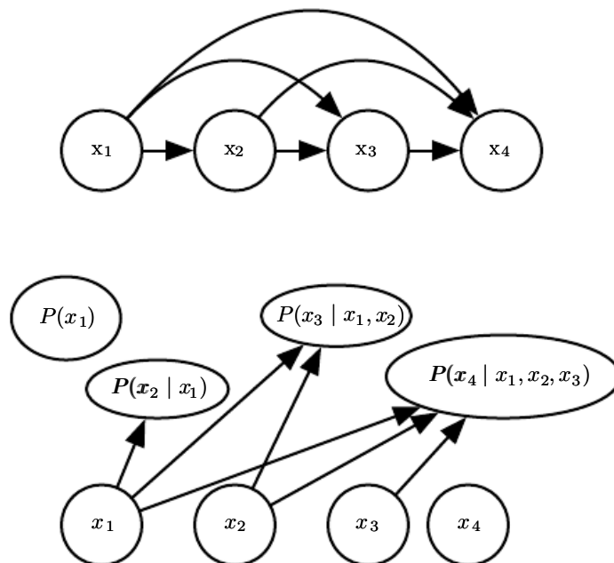
Figure 20.8: A fully visible belief network predicts the i -th variable from the i - 1 previous ones. (Top)The directed graphical model for an FVBN. (Bottom)Corresponding computational graph for the logistic FVBN, where each prediction is made by a linear predictor.
